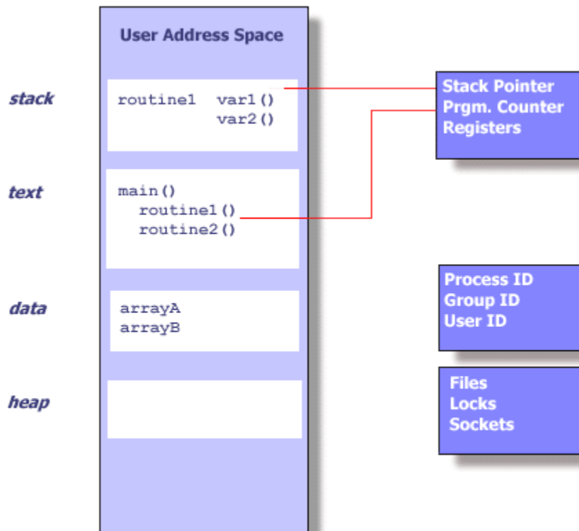
UNIX PROCESS
