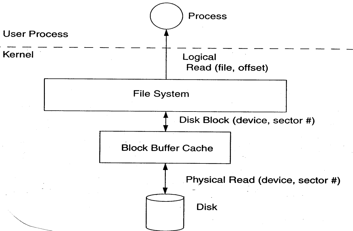
The Old-Style Buffer Cache
